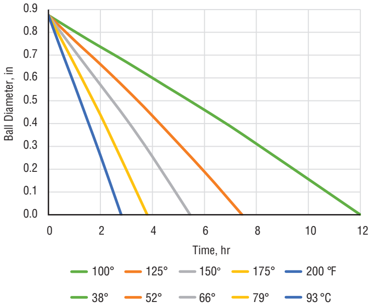
Dissolvability Curves in 2% Potassium Chloride (KCL) PS-MT 0.875 in [22 mm]
