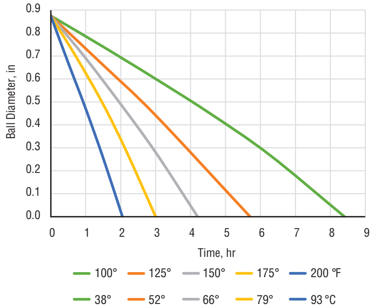
Dissolvability Curves in 15% Hydrochloric Acid (HCl) PS-MT 0.875 in [22 mm]
